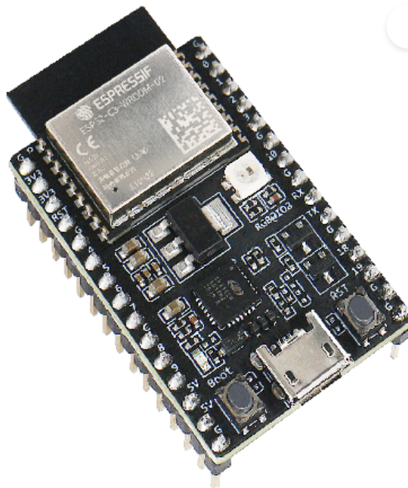
ESP32-C3-DevKitC-02
