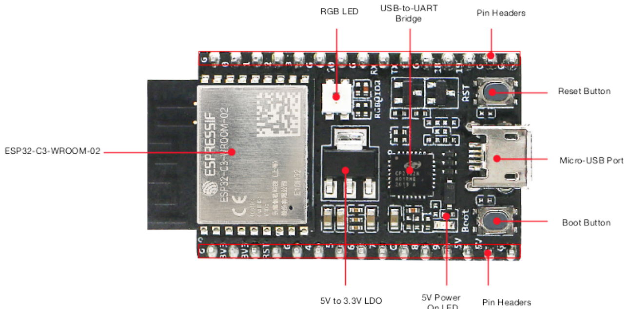
ESP32-C3-DevKitC-02 - front
